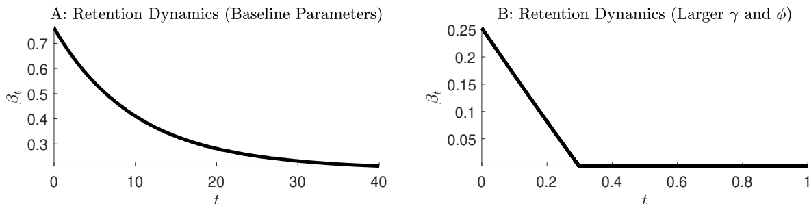
Figure 3: Implementation of the optimal contract and per unit value of the loan. Panel A uses our baseline parameters and Panel B sets \gamma = 0.12 and \phi = 65 .
