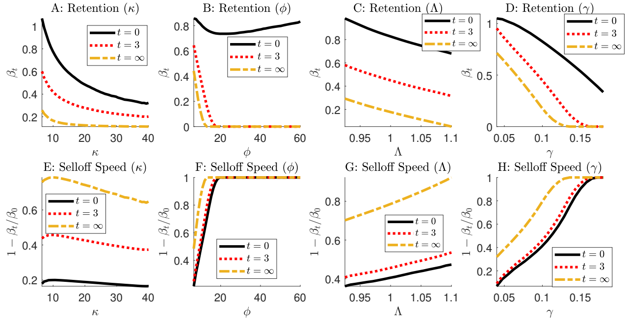
Figure B.3: Retention and dynamics with finite maturity. We use our baseline parameters and \delta = 0.2 .
